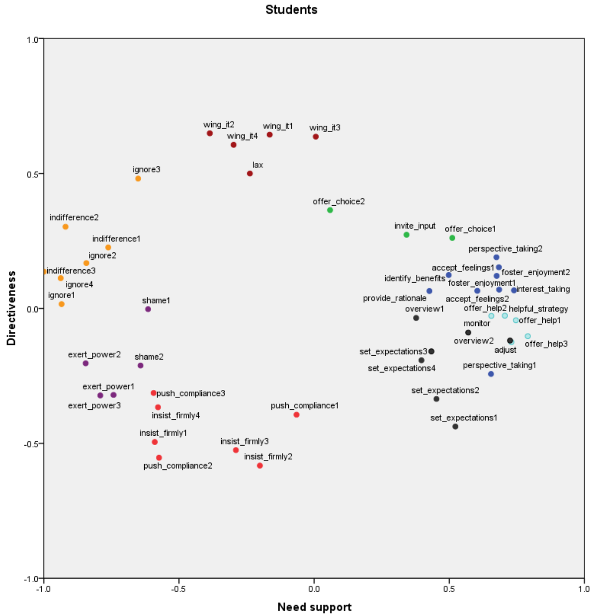
Two-dimensional Configuration of the SIS Items among Students (Samples 4 and 5)
