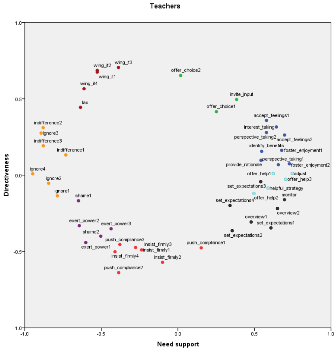
Two-dimensional Configuration of the SIS Items among Teachers (Samples 1, 2, 3, and 5)
